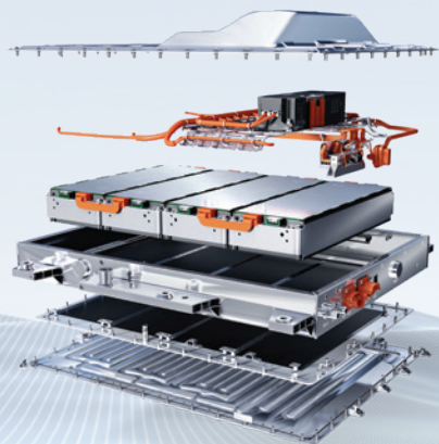
Ternary Lithium Battery
